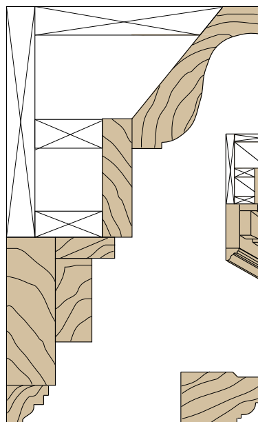
1 Cornice
