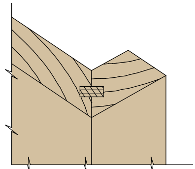
Splined Miter Joint Figure: RG-1126
