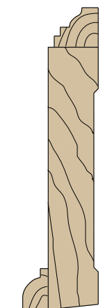
3 3-piece Base
