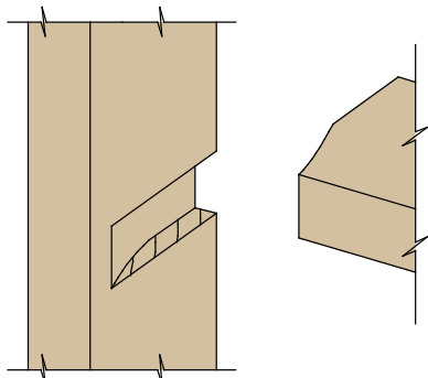
Dado, Blind Or Stopped Joint Figure: RG-124
