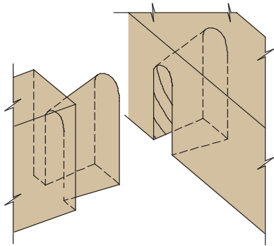
Blind Dovetail Joint Figure: RG-121
