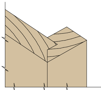
Shoulder Miter Joint Figure: RG-127
